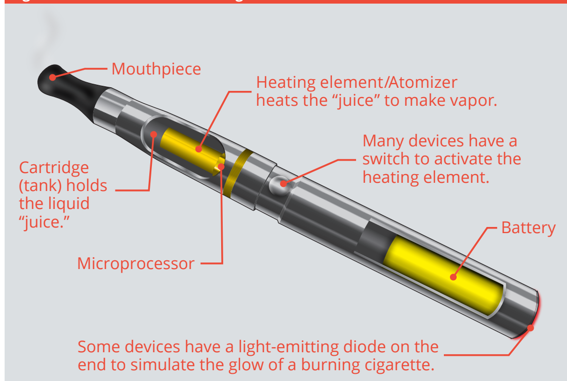
Figure 2. Parts of an electronic cigarette.
